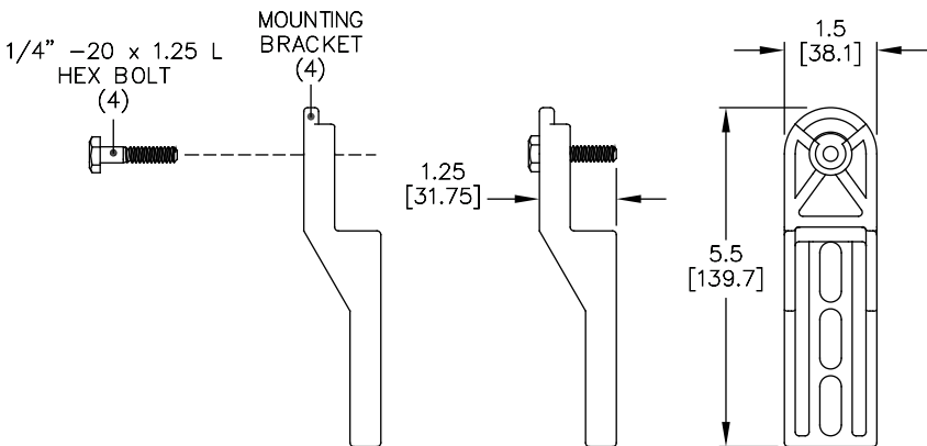
Mounting Brackets
